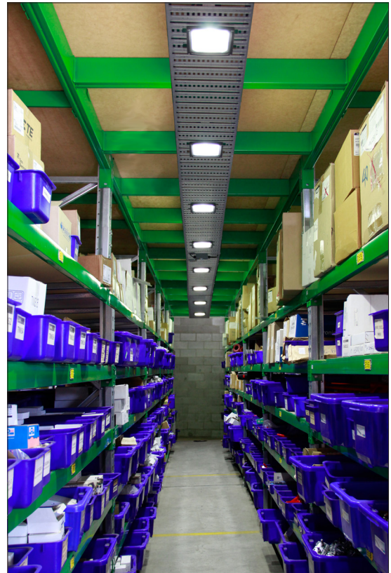
After: Low level picking isle illuminated by ECOLight LEDFL11 floodlights mounted in cable tray and operated by motion sensor to save even more energy.
