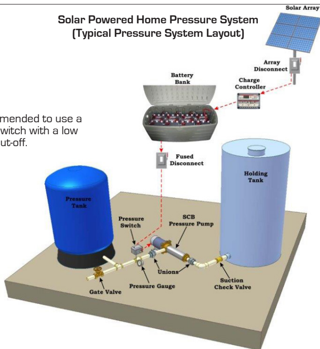
Surface Pressure Pump showing Solar Panels and Tanks
