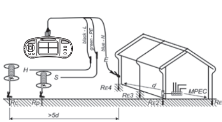
Circuits for three-wire measurement
