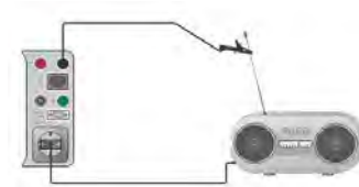
Substitute leakage test for Class II device
