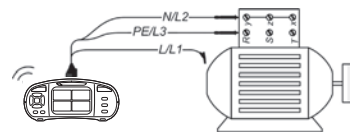
Test circuit for continuous resistance measurement
