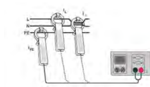
Current measurement with current clamps
