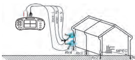
Circuit for two clamps measurement
