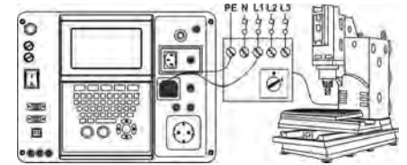
Discharge time test
